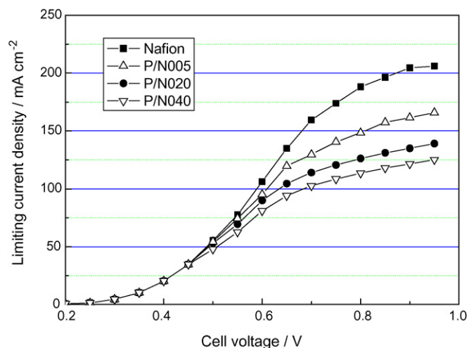
Fig. 4. Methanol permeation measurement of PPy/Nafion composite membranes at 80 °C in DMFC configuration.
